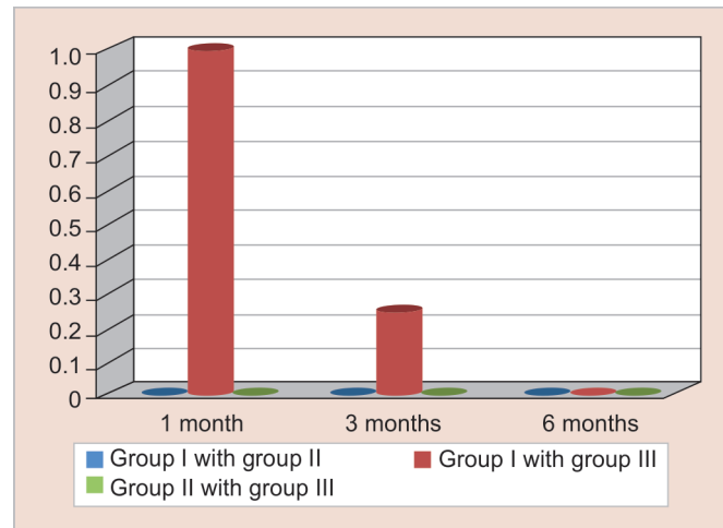
Fig. 5: The comparison of probability values based on Bonferroni multiple comparison test at various intervals of the study. (Intercomparison)
